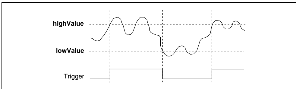
Figure 2-7. ND_HIGH_HYSTERESIS
