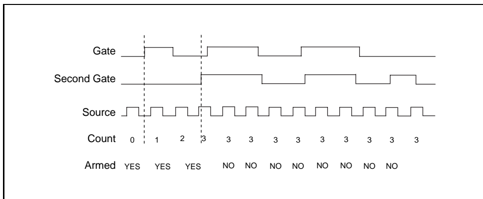
Figure 2-18. Start-Stop Measurement
