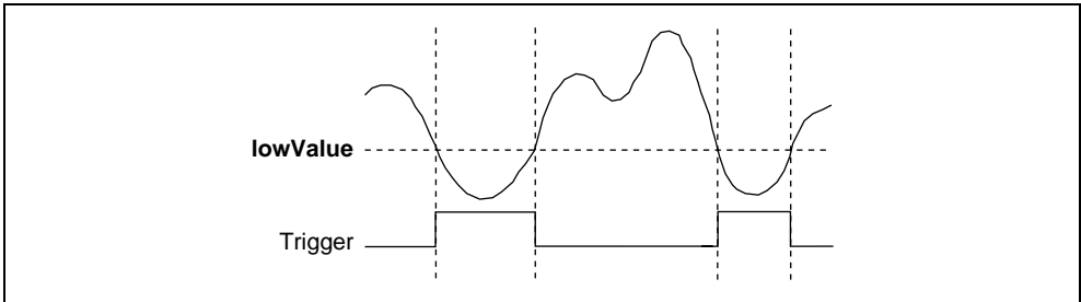
Figure 2-4. ND_BELOW_LOW_LEVEL
