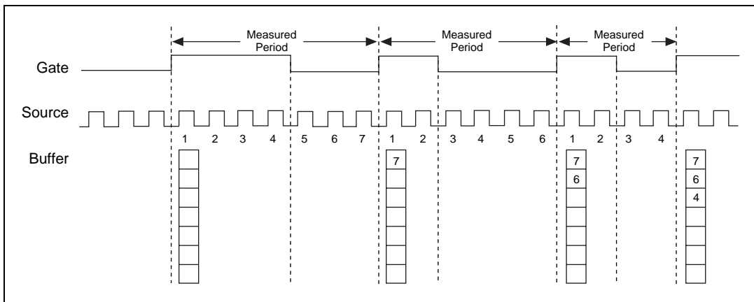
Figure 2-24. Buffered Event Counting
