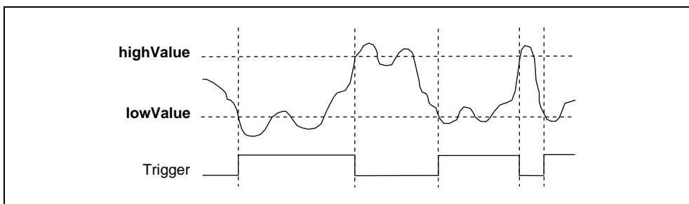
Figure 2-8. ND_LOW_HYSTERESIS
