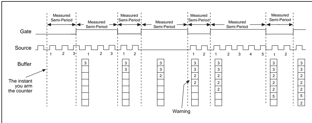
Figure 2-28. Buffered Semi-Period Measurement when No Source Edges Are Present between Gate Edges
